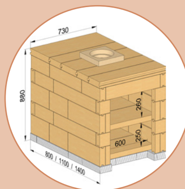
REMUS Duo
